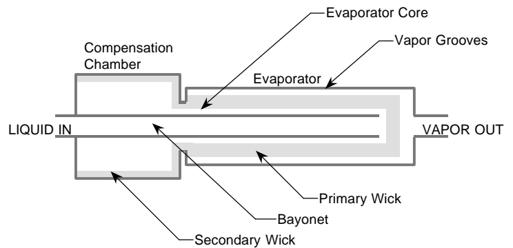
Figure 1: Depiction of LHP Evaporator
