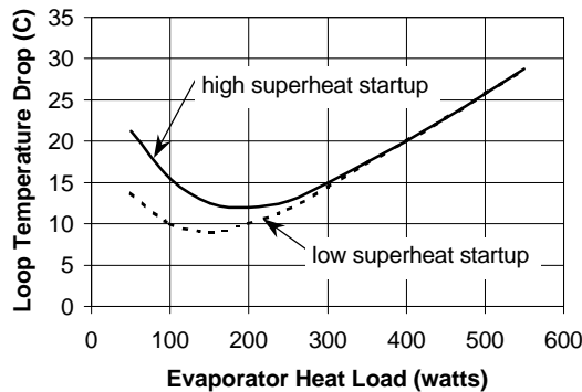
Figure 2: Phase Dependent Operational Curves of an LHP (NRL Loop Test Data, Reference 1)
