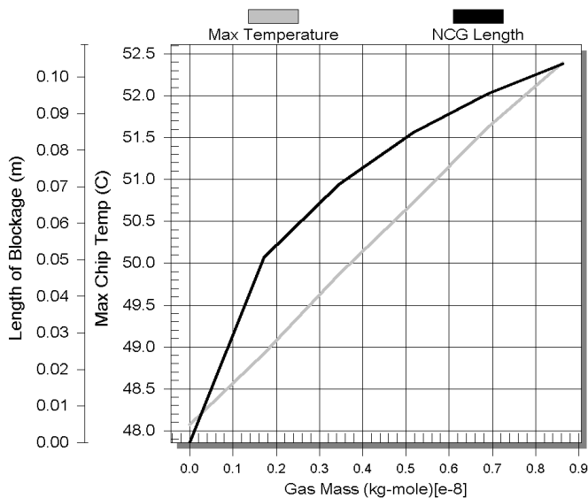
Figure 4: Effect of Degradation via NCG Generation
