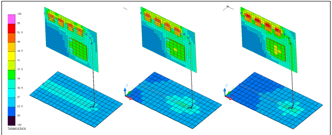
Figure 3: Parametric Study of Heat Pipe Degradation from Zero NCG (left) to 8.5 \times 10^{-9} kg-mole (right)
