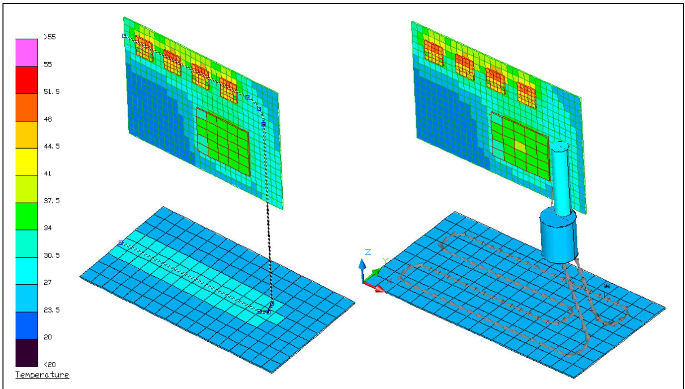
Figure 5: LHP Replacement System with Serpentine Condenser (Prior Heat Pipe Solution Shown at Left)
