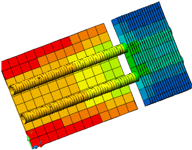
Figure 2: Chip-to-Fin Heat Pipes Modeled as a 2D Cylindrical Shell Attached to Finite Difference Plates
