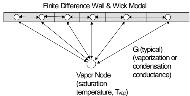
Figure 1: System-level Network Model of a Heat Pipe
